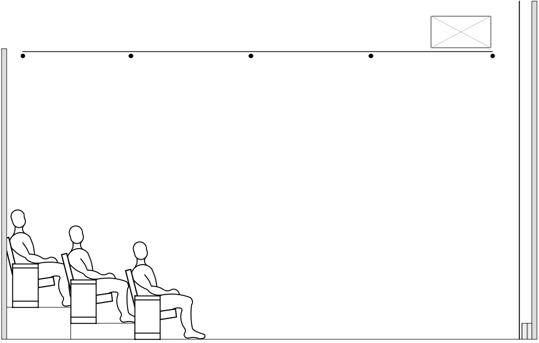
CENTERLINE SECTION
